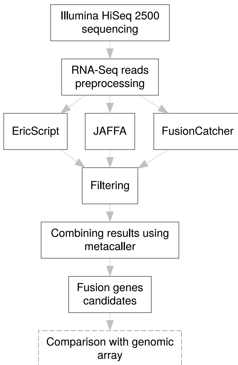
Figure 3 Pipeline design for fusion gene identification. Schematic overview of RNA-Seq fusion gene identification pipeline summarizes all steps of the procedure. Comparison with results of the genomic arrays is an optional manual step, independent on the pipeline, which can serve as a secondary confirmation of the results.
