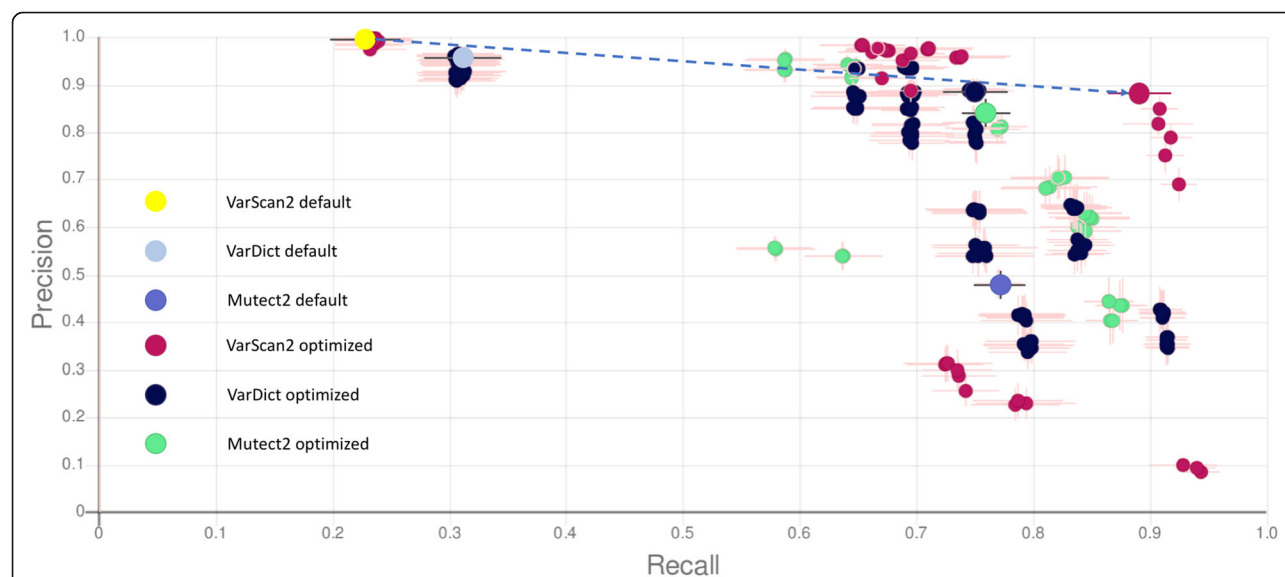
Fig. 2 Each dot represents an arithmetic mean of recall (X-axis) and precision (Y-axis) for one pipeline configuration calculated based on repeated random sub-sampling of 3 input datasets (220 samples). The crosshair lines show the standard deviation of the respective results across the sub-sampled sets. Individual variant callers (Mutect2, VarDict and VarScan2) are colour coded with a distinguished default setting for each. The default settings and the best performing configurations for each variant caller are also enlarged. Based on our experiment, the largest variant calling improvement (2.36× higher F-measure compared to default settings, highlighted by an arrow) and also the highest overall recall, precision, precision-recall, and F-measure were registered for VarScan2. In case of VarDict, a significant improvement in variant detection, mainly for recall (2.42×) was observed. The optimization effect on Mutect2 had a great effect on increasing the precision (1.74×). Although the F-measure after optimization did not reach as high values as VarScan2 and VarDict, Mutect2’s default setting provided the best results, mainly in a sense of recall
