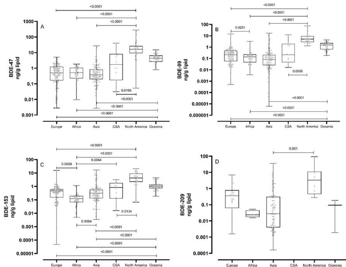
Figure 3. Box-and-whiskers (horizontal lines are medians, 95% confidence intervals, minima, and maxima) of individual PBDE congeners: A) BDE-47, B) BDE-99, C) BDE-153, and D) BDE-209 concentrations in different regions (CSA= Central- and South America and the Caribbean), in breast milk data collected after year 2000. Non-parametric ANOVA tests (Kruskal-Wallis with Dunn's post-tests) were conducted to determine significant differences. From van der Schyff et al. (2023a).
