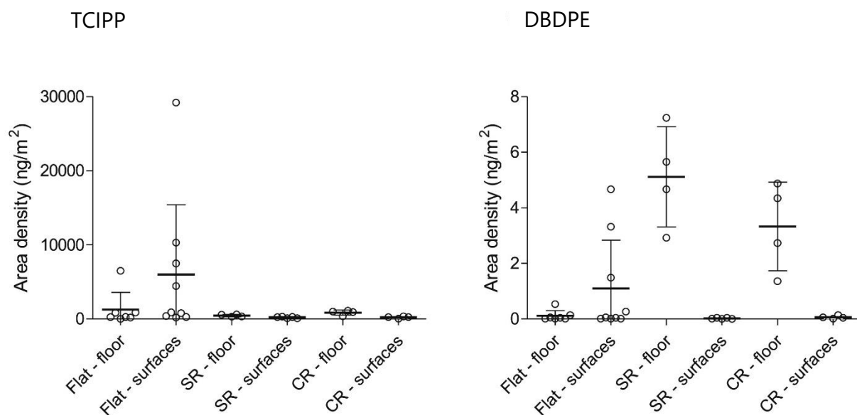
Figure 9 Area density of TCIPP and DBDPE in a flat and a classroom floor dust and wipe samples. Horizontal lines show mean and whiskers show standard deviation. Extracted from Jilkova et al. (2018). SR refers to Seminar room and CR refers to Computer Room.
