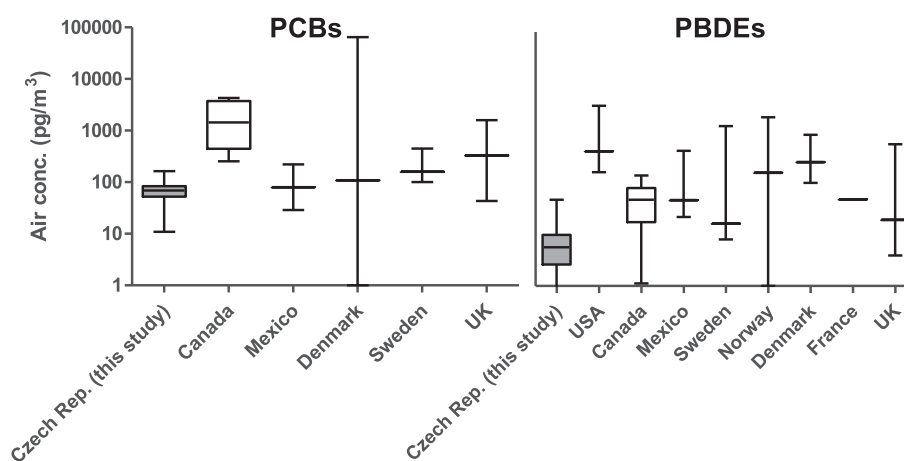
Fig. 1. Comparison between medians and range of indoor air concentrations of PCBs and PBDEs measured in this study with previously published concentrations from Canada (Zhang et al., 2011), USA (Allen et al., 2007), Mexico (Bohlin et al., 2008), Sweden (Bjorklund et al., 2012; Bohlin et al., 2008), Norway (Cequier et al., 2014), Denmark (Frederiksen et al., 2012; Vorkamp et al., 2011), France (Alliot et al., 2014) and UK (Bohlin et al., 2008; Harrad et al., 2006).
