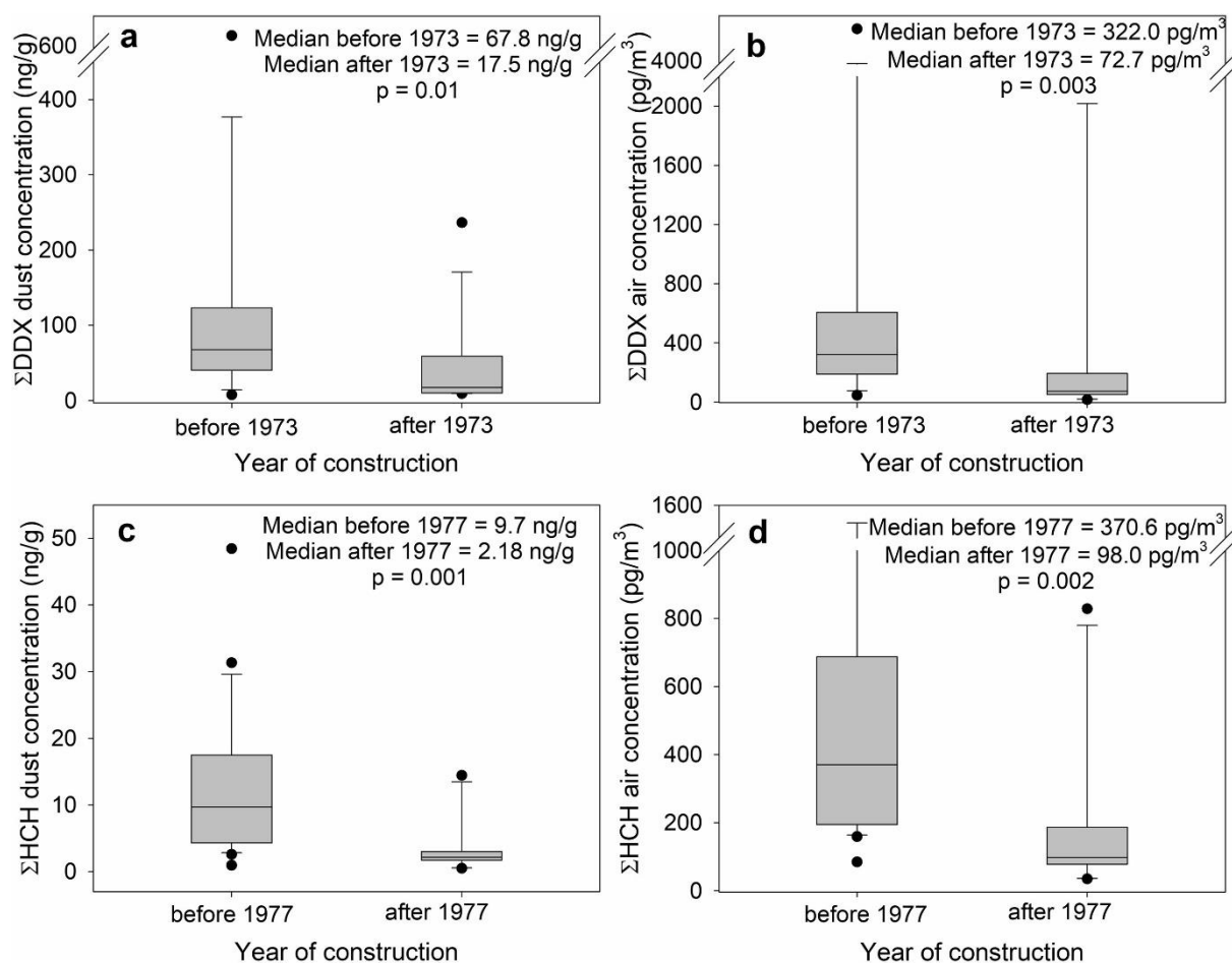
Figure 7 Differences in indoor dust and air concentrations of \Sigma DDX (a and b) and \Sigma HCH (c and d) measured in homes built before ( n = 18 for \Sigma DDX, n = 22 for \Sigma HCH) and after ( n = 14 for \Sigma DDX, n = 10 for \Sigma HCH) OCPs controls were implemented in Czechoslovakia. Excerpted from Demirtepe et al. (2019).
