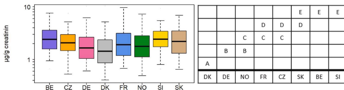
Figure 5 Box plot of creatinine-adjusted concentrations of diphenyl phosphate (DPHP), a metabolite of TPHP, for Belgium (BE), Czech Republic (CZ), Germany (DE), Denmark, France (FR), Norway (NO), Slovenia (SI), and Slovakia (SK). The box indicates median, 25% and 75% percentiles. Whiskers indicate 5% and 95% percentiles. From van der Schyff et al. (2023b). The table on the right groups the countries according to where significant differences exist between urinary concentrations, e.g., DK is lower than all other countries, while DE and NO are similar concentrations.
