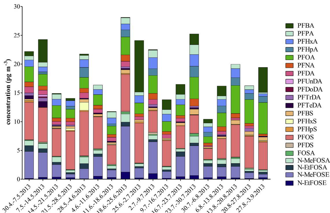
Fig. 1. Gas + particle phase concentrations ( \text{pg m}^{-3} ) of individual PFASs compounds in outdoor air measured by active air sampler ( \text{OUT}_{\text{totalAAS}} samples) during outdoor PAS calibration.
