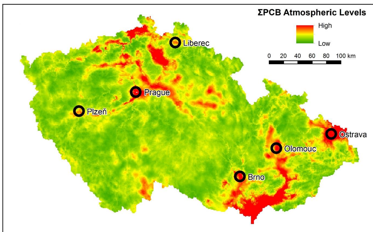
Figure 8 Application of the LUR models across all of Czechia, indicating the estimated gradient of low to high atmospheric levels of \Sigma_7\text{PCB} , ( R^2 = 0.62 ). Cities with population > 100,000 are indicated on the map. From White et al. (2021)
