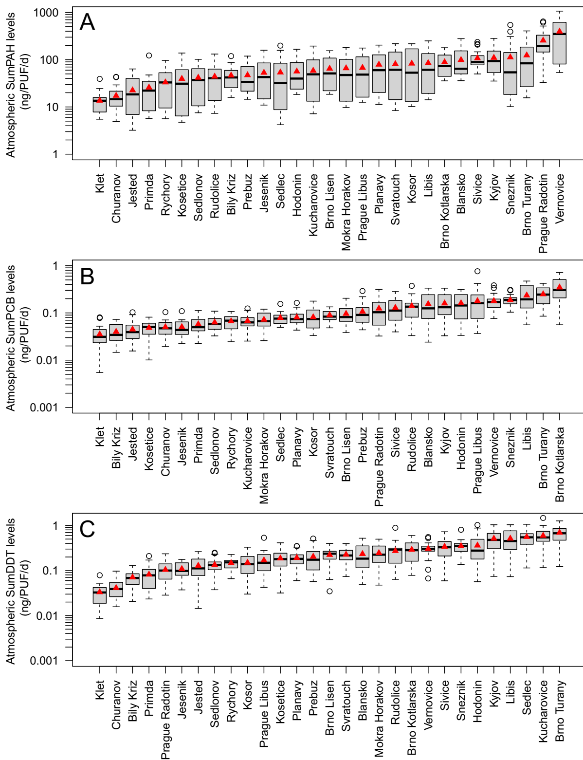
Fig. 2. Log-boxplots of atmospheric levels (ng per PUF disk per day) of A) \sum_{14} PAH; B) \sum_{7} PCB; and C) \sum_{6} DDT. Levels measured monthly (28-d) by passive sampling over a two-year period (July 2015–June 2017) at 29 sites across Czechia ( n = 24 –26 at each site). Boxplots depict the interquartile range (IQR): box upper limit is the 75th percentile, horizontal line is the 50th percentile (median), box lower limit is the 25th percentile; whiskers above and below depict 1.5 x IQR; data points outside this range (outliers) are depicted as hollow circles. Sites are listed in order of increasing average level (depicted by triangles).
