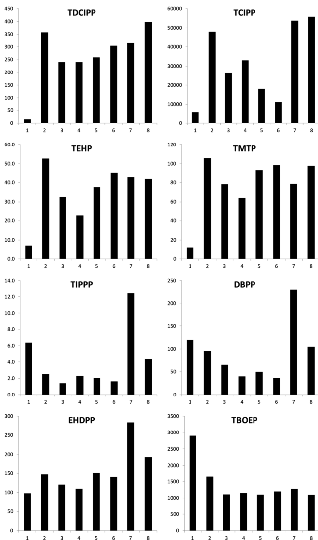
Figure 5. Changes in air concentrations ( \text{pg m}^{-3} ) of OPEs over time in computer room. Sample numbers ( x -axis) correspond to the sampling events identified in Figure 1.
