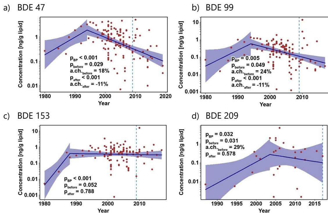
Figure 2 Results of breakpoint analysis for PBDEs in human milk for Europe for individual PBDE congeners: BDE-47, BDE-99, BDE-153 and BDE-209. The shaded area indicates 95th percent confidence interval. The dotted blue line indicates when regulation was implemented by the Stockholm Convention (2009: BDE-47, -99, and -153; 2019: BDE-209). From van der Schyff et al. (2023a).
